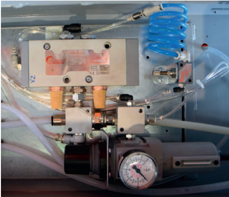
Some Bonesi Pneumatik products on a Filma machine.
