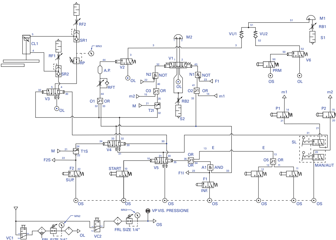
Bonesi Pneumatik has co-operated with Filma to develop the diagram of the wrapping machine of palletized loads with stretch film, totally pneumatic.
