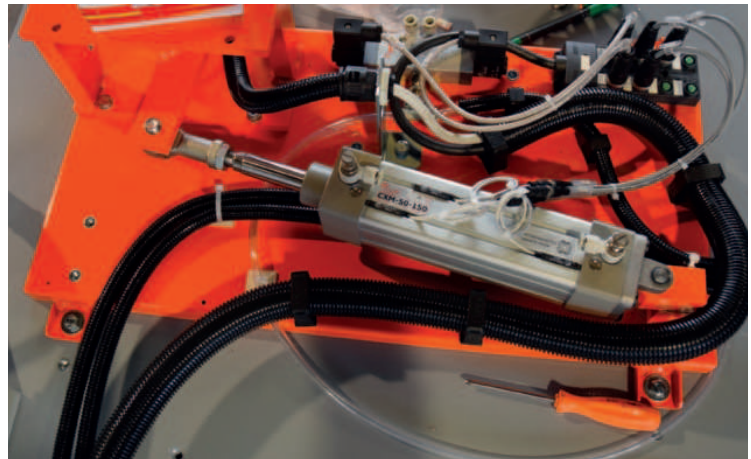
View of Bonesi Pneumatik ISO 15552 cylinder series CXM used on a tensioning group of stretch film.
